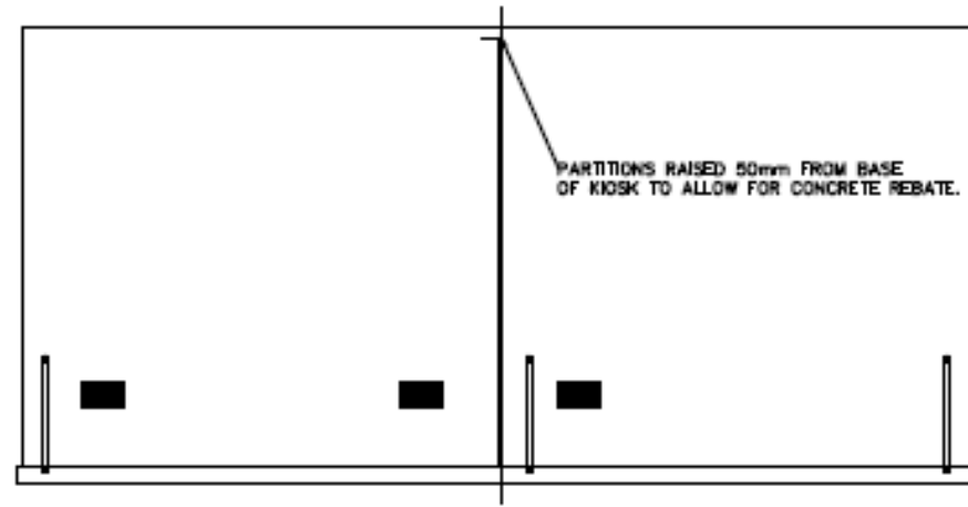
REAR VIEW
