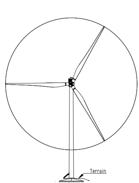
Blade in Horizontal position
